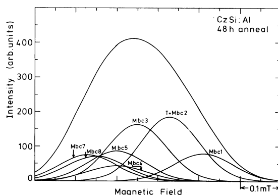
Fig. 2. Multispecies character of the Si-NL10 thermal donor as unraveled by the FStENDOR technique for an Al-doped Cz-Si sample following 470°C/48 h annealing. As can be seen, at least seven different components contributing to the overall EPR line could be traced.
