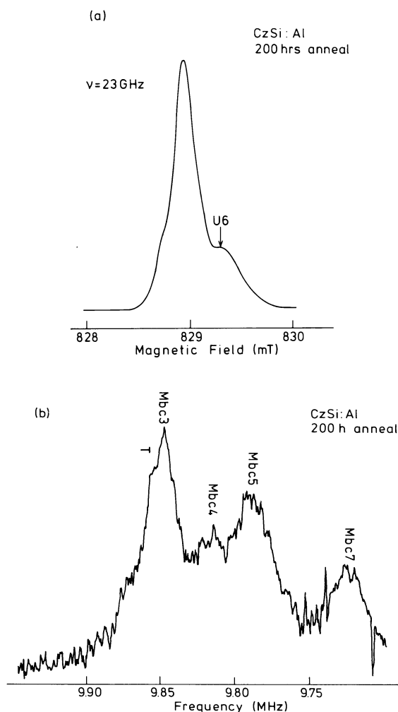
Fig. 3. Si-NL10 EPR (a) and ENDOR (b) spectra of a Cz-Si:Al sample annealed at 470°C for 200 h obtained for 23 GHz microwave frequency. Magnetic field is along the [0 1 1] crystallographic direction. The same sample was used for the HF-EPR experiment (see fig. 4). The ENDOR spectrum was measured at the U6 high symmetry point. The individual resonance lines are marked according to their different species of origin.
