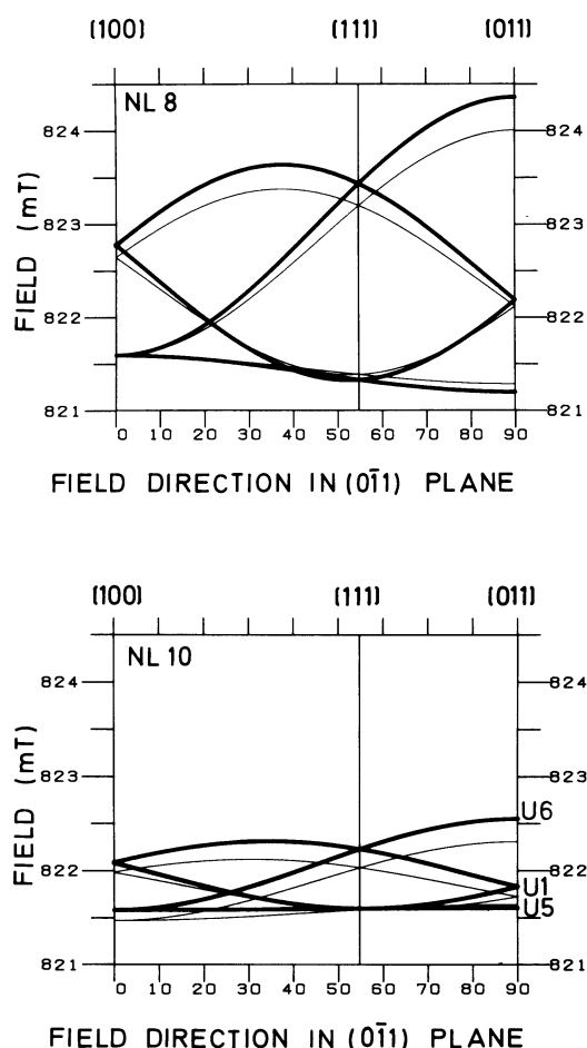
Fig. 1. g -shifting effect as observed by standard EPR technique (23 GHz) for (a) Si-NL8 and (b) Si-NL10 TD-related spectra. The thick and thin lines correspond to annealing at 470°C for 10 and 100 h, respectively. For the Si-NL10 spectrum the U1, U5, and U6 high symmetry points are marked.
