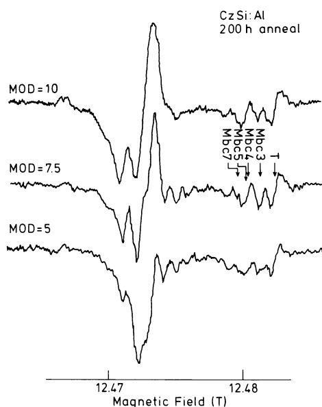
Fig. 4. HF-EPR spectrum of a Cz-Si:Al sample heat-treated for 200 h at 470°C. The frequency is 349 GHz and the magnetic field (along the [011] crystallographic direction) is in the 12 T range. The well-resolved EPR lines corresponding to individual Si-NL10 species are indicated. Three spectra as obtained for three different field modulation values are shown.
